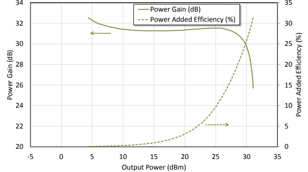
Power Gain (dB) and Power Added Efficiency (%) vs. Output Power (dBm) @ 20.62GHz, V_d = 5\text{V} , I_d = 650\text{mA}
