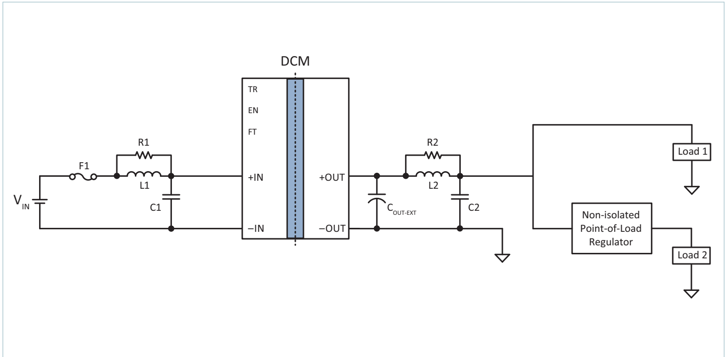
Typical Application 1: Single DCM3623x50T0680y7z, to a non-isolated regulator, and direct to load
