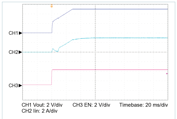
Figure 14 — Startup from EN, V_{IN} = 30\text{ V} , C_{OUT\_EXT} = 10000\ \mu\text{F} , R_{LOAD} = 0.313\ \Omega
