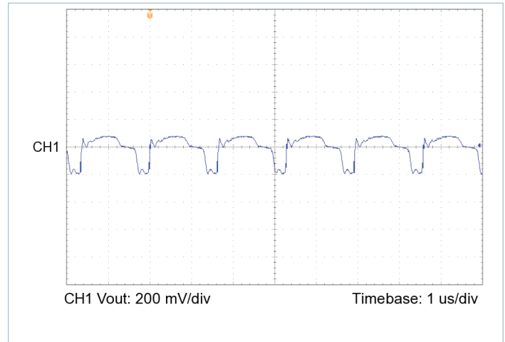
Figure 16 — Output voltage ripple, V_{IN} = 30\text{ V} , V_{OUT} = 5.0\text{ V} , C_{OUT\_EXT} = 1000\ \mu\text{F} , R_{LOAD} = 0.313\ \Omega
