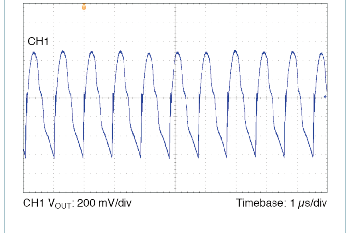
Figure 16 — Output voltage ripple, V_{IN} = 300\text{ V} , V_{OUT} = 48.0\text{ V} , C_{OUT\_EXT} = 220\ \mu\text{F} , R_{LOAD} = 4.571\ \Omega
