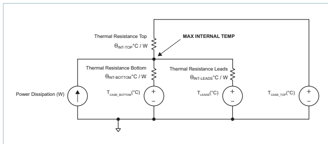
Figure 17 — Double side cooling and leads thermal model
