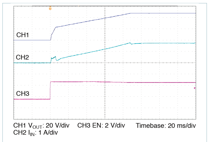
Figure 14 — Startup from EN, V_{IN} = 300\text{ V} , C_{OUT\_EXT} = 2200\ \mu\text{F} , R_{LOAD} = 4.571\ \Omega
