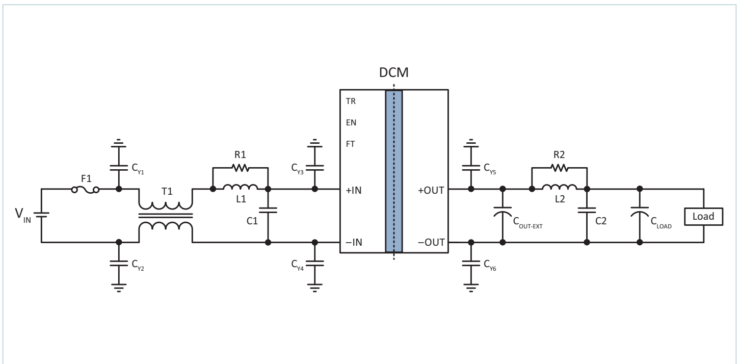
Typical Application 2: Single DCM4623xD2H53E0y7z with common- and differential-mode input filters
