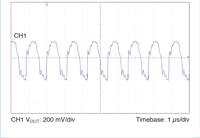
Figure 16 — Output voltage ripple, V_{IN} = 270\text{ V} , V_{OUT} = 15.0\text{ V} , C_{OUT\_EXT} = 680\ \mu\text{F} , R_{LOAD} = 0.449\ \Omega
