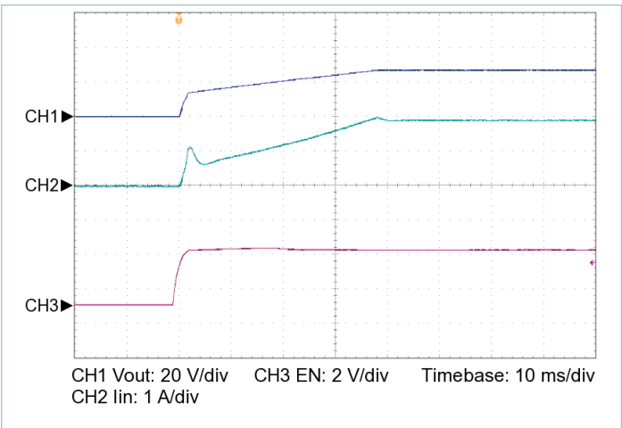
Figure 17 — Startup from EN, V_{IN} = 270\text{ V} , C_{OUT\_EXT} = 2000\ \mu\text{F} , R_{LOAD} = 1.568\ \Omega
