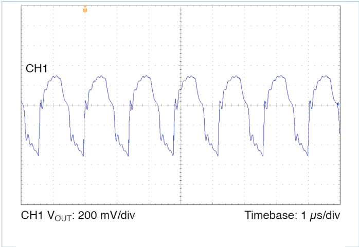
Figure 19 — Output voltage ripple, V_{IN} = 270\text{ V} , V_{OUT} = 28.0\text{ V} , C_{OUT\_EXT} = 200\ \mu\text{F} , R_{LOAD} = 1.568\ \Omega
