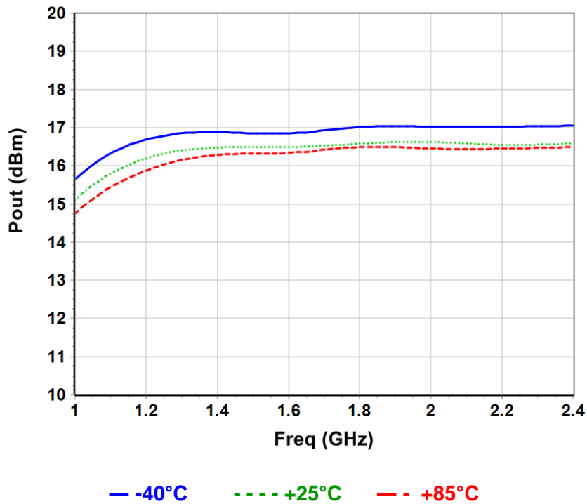
Output power @ 1dB comp. versus Frequency
