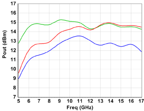
P 1dB versus Frequency and Id
