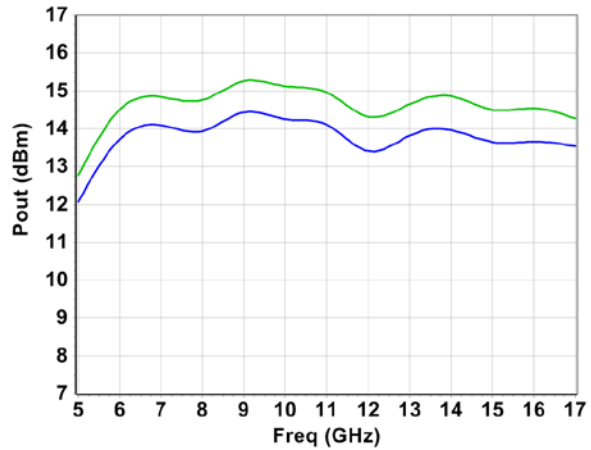
P 1dB versus Frequency and Vd
