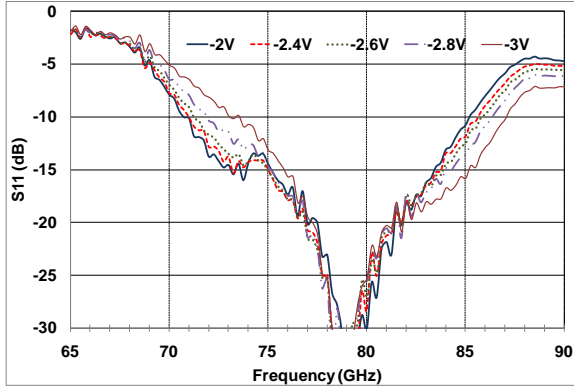
Input Return loss versus vg voltage
