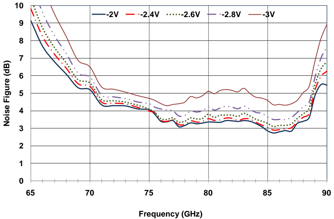
Noise Figure versus Vg voltage
