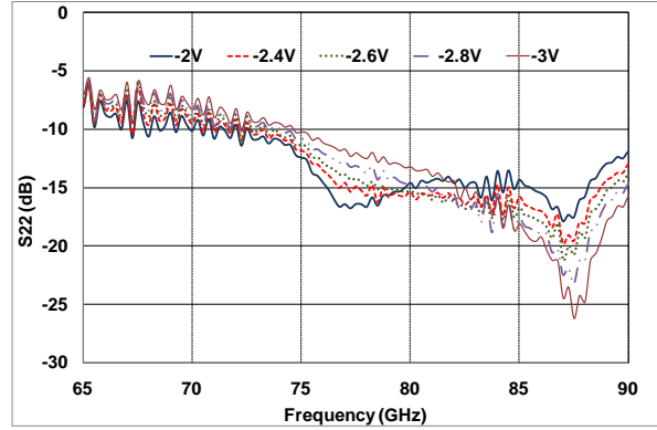
Output Return loss versus vg Voltage
