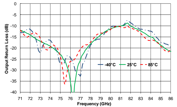
Output Return Loss versus Temperature
