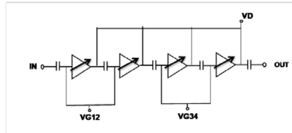
Functional diagram
