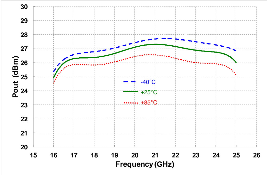
Output Power @ 1dB Comp versus Frequency and Temperature
