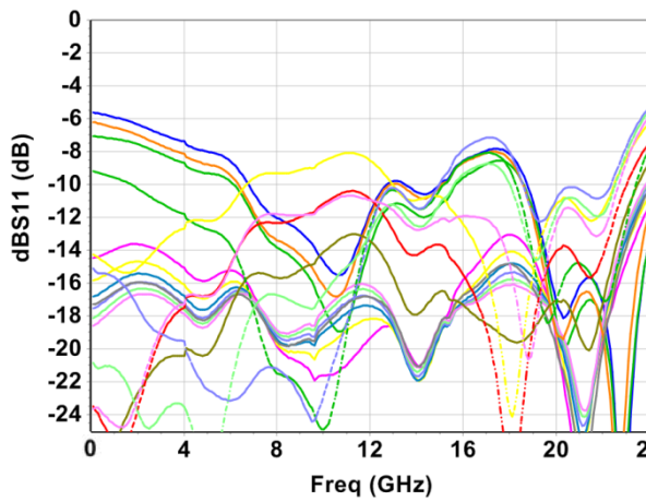
Input Return Loss versus Frequency and Gain Control Voltage
