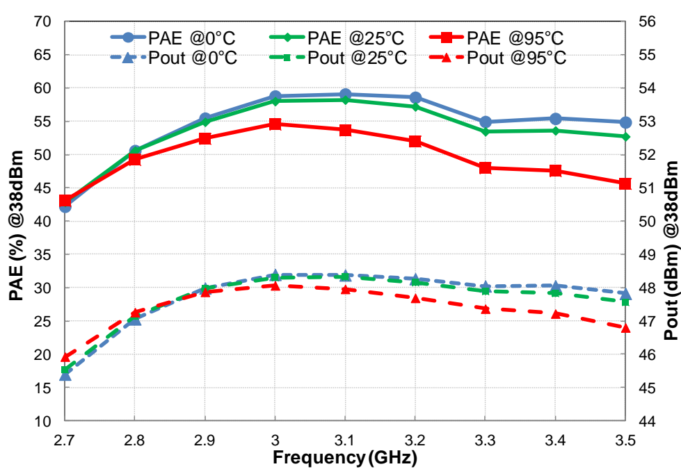
Pout & PAE versus Frequency and Temperature @ Pin=38dBm
