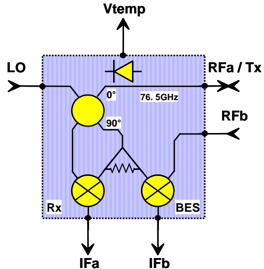
Transmitter/Receiver block diagram
