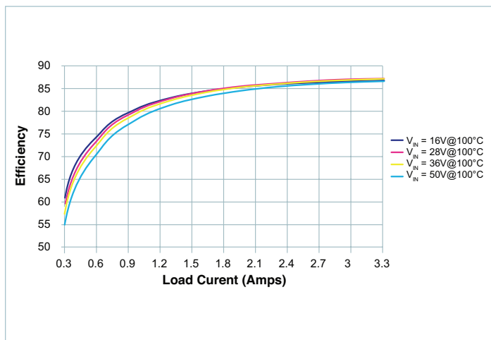
Figure 31 — Conversion efficiency
