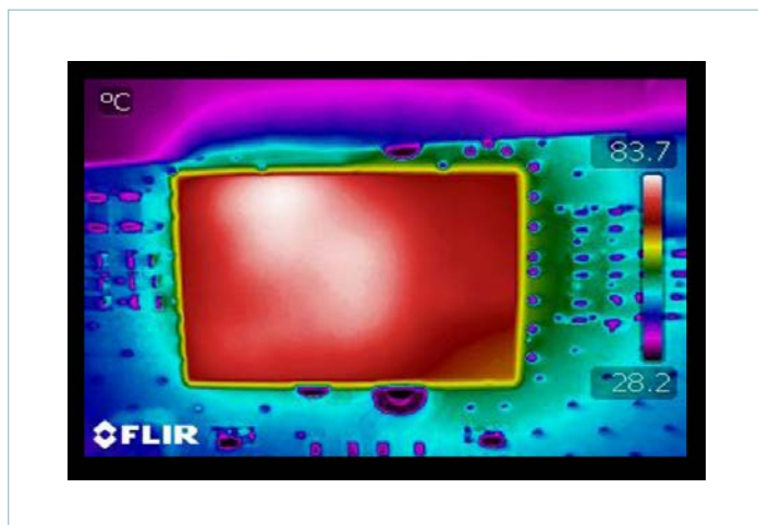
Figure 30 — Thermal image ( V_{IN} = 28V , I_{OUT} = 4.2A , CR, OLFM evaluation PCB)
