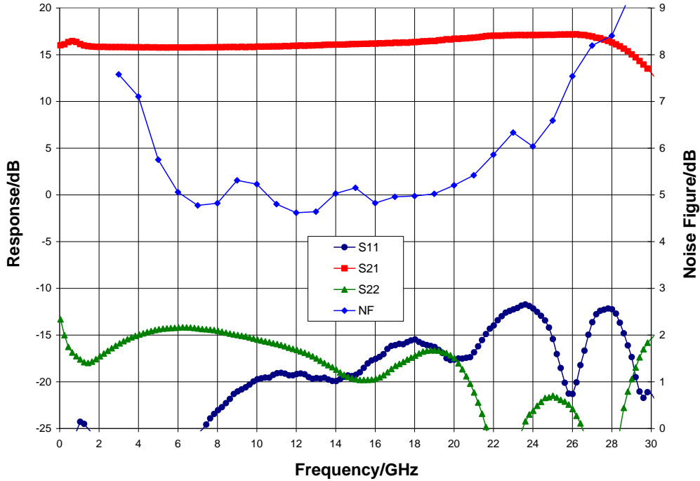
Broadband Performance, V_{dd} = 5.0\text{ V} , V_{gg} = 3.0\text{ V} , I_{dd} = 74\text{ mA} , T_A = 25^\circ\text{ C}
