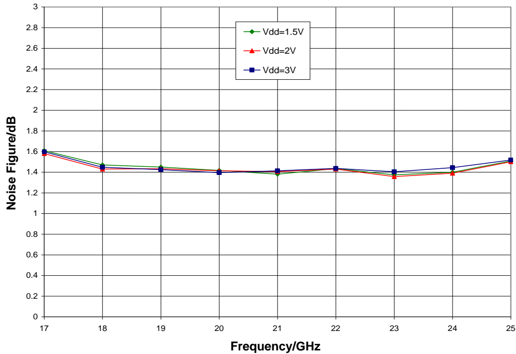
Noise Figure vs. V_{dd} , V_{gg} = 1.5\text{ V} , T_A = 25^\circ\text{C}
