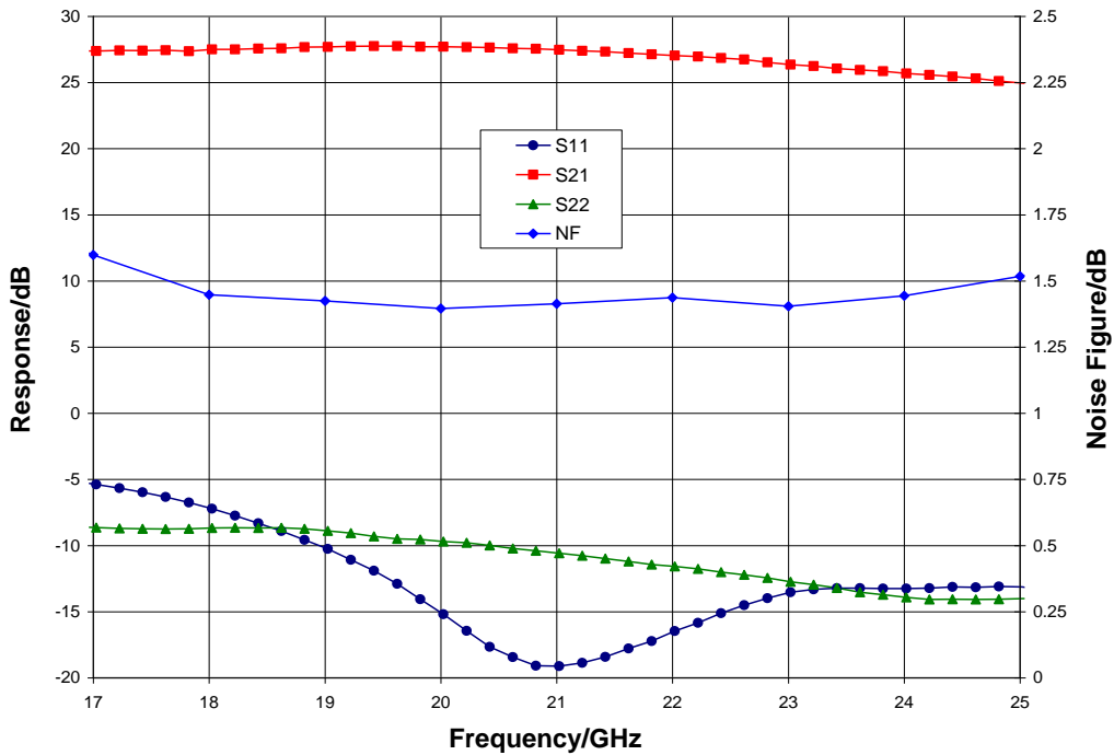
Narrow-band Performance, V_{dd} = 3.0\text{ V} , V_{gg} = 1.5\text{ V} , I_{dd} = 27\text{ mA} , T_A = 25^\circ\text{ C}
