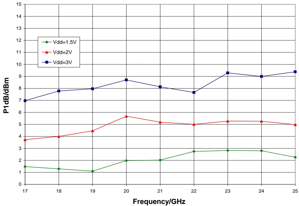
P1dB vs. V_{dd} , V_{gg} = 1.5\text{ V} , T_A = 25^\circ\text{ C}
