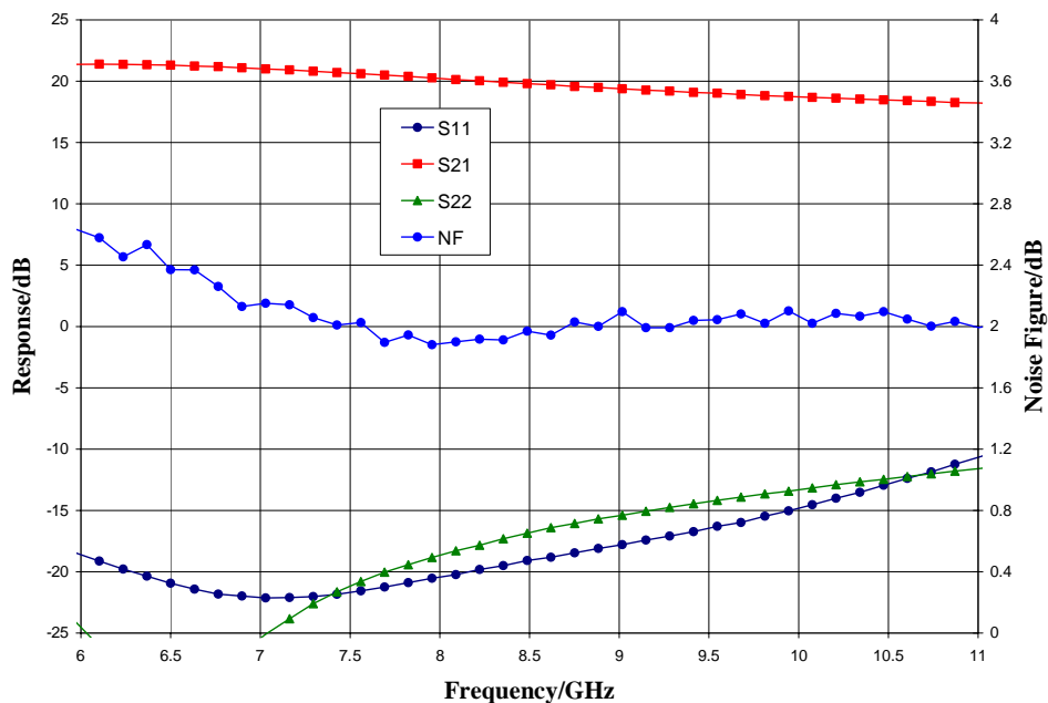
Narrow-band Performance, V_{dd} = 5.0\text{ V} , T_A = 25\text{ }^\circ\text{C}
