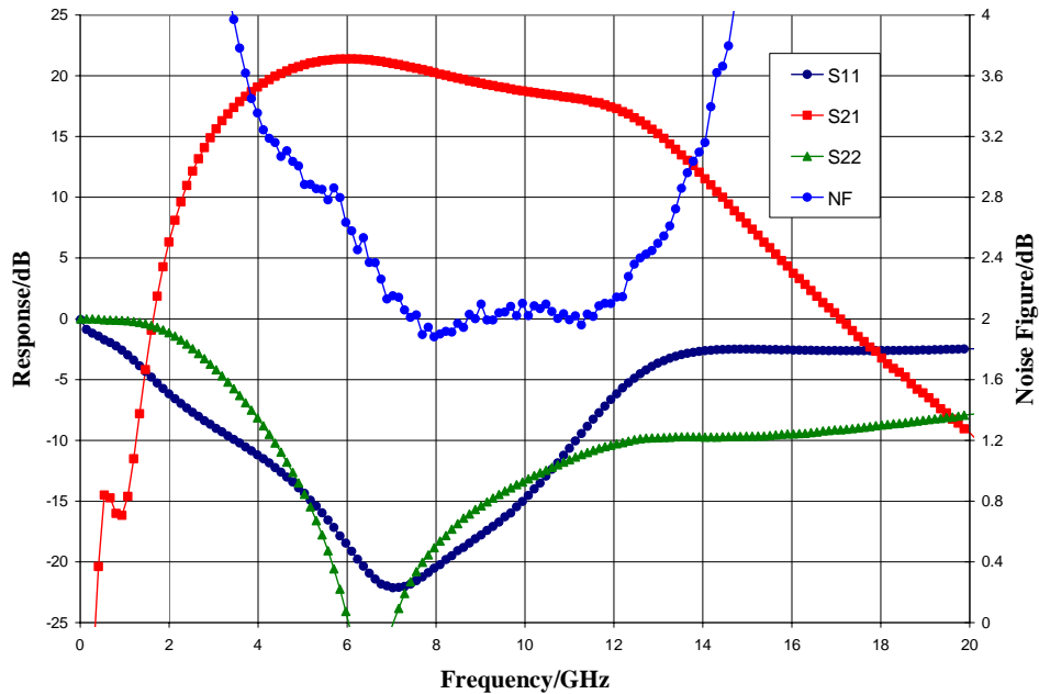
Broadband Performance, V_{dd} = 5.0\text{ V} , T_A = 25\text{ }^\circ\text{C}
