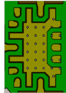
MOUNTING DETAIL
