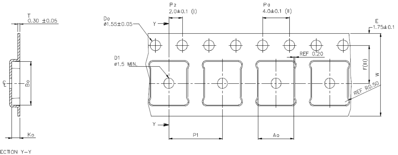
SECTION Y-Y
