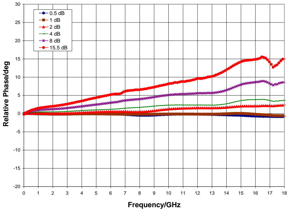
Relative Phase versus Frequency, T_A = 25\text{ }^\circ\text{C}
