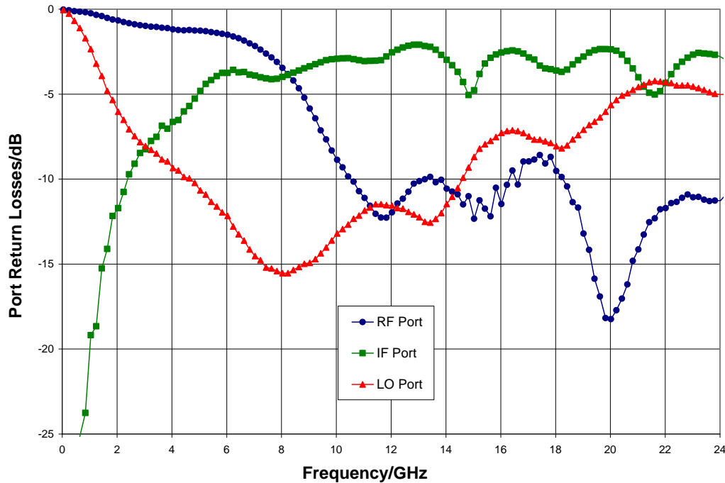
Return Loss, LO = +2 dBm, T A = 25 °C
