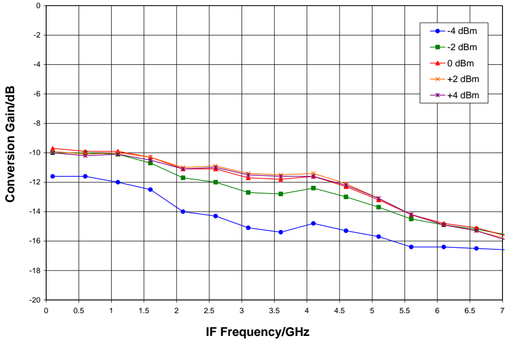
IF Bandwidth, LO = +2 dBm, T A = 25 °C
