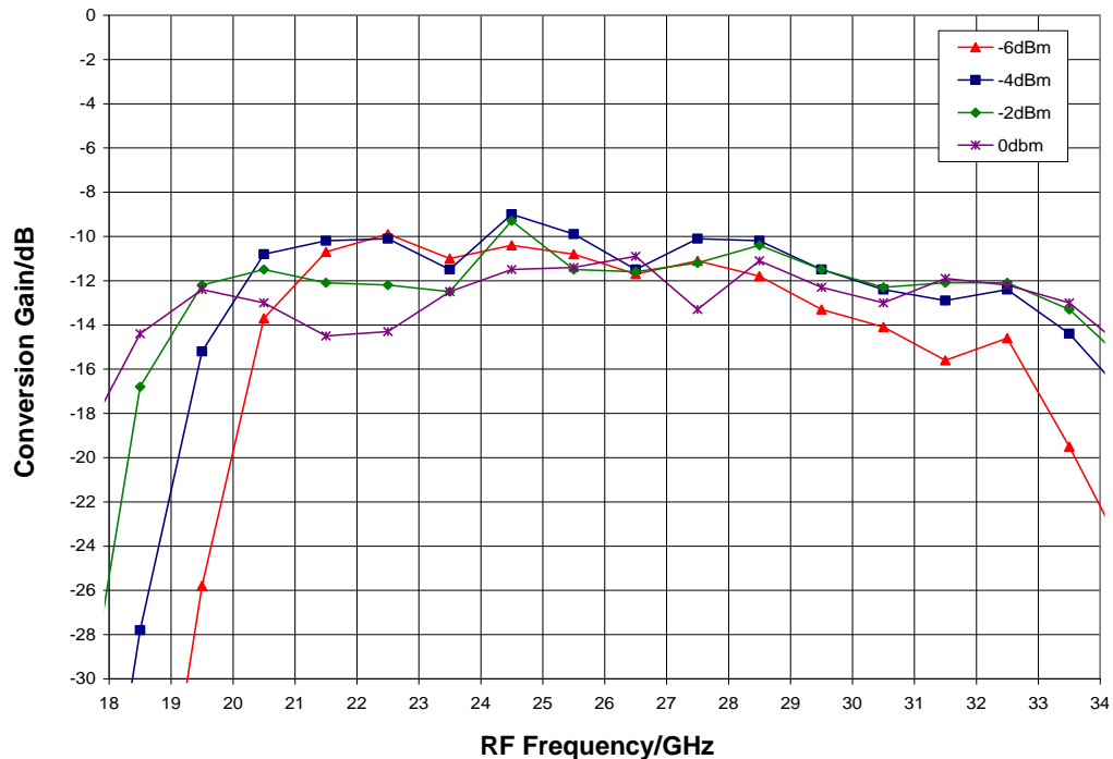
Upconverter Performance, Conversion Gain vs. LO Drive, T_A = 25\text{ }^\circ\text{C}
