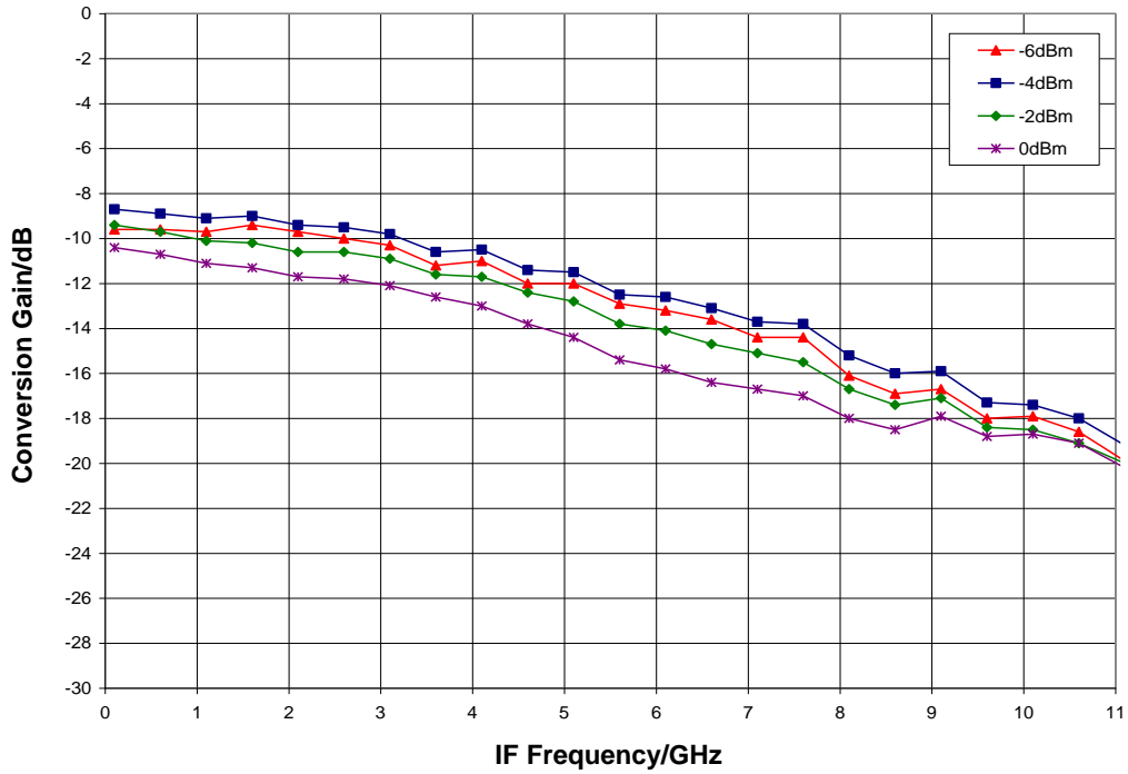
IF Bandwidth vs. LO Drive, T_A = 25\text{ }^\circ\text{C}
