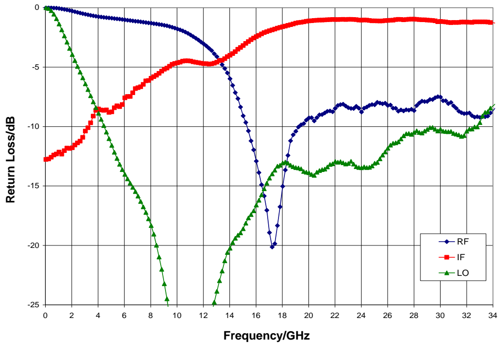
Return Loss, LO = -4 dBm, T A = 25 °C
