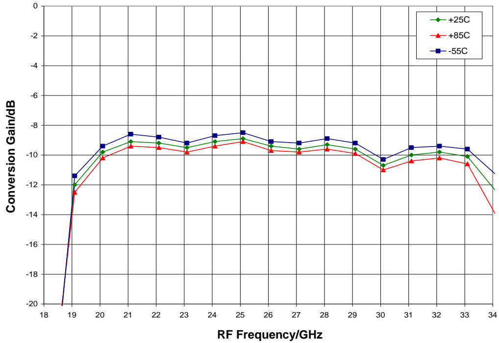
Conversion Gain vs. Temperature, LO = -4 dBm, IF = 100 MHz USB
