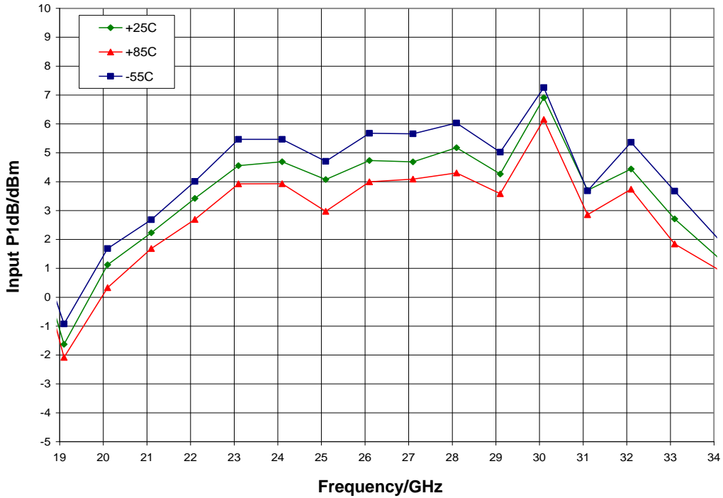
Input P1dB vs. Temperature, LO = -4 dBm, T A = 25 °C
