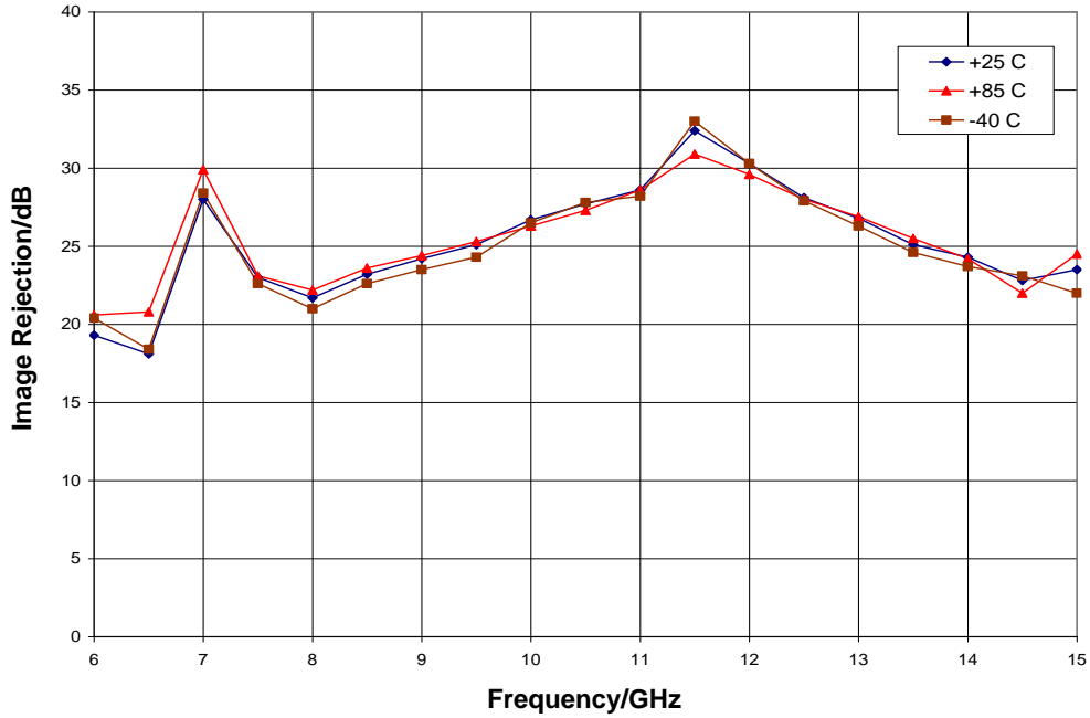
Image Rejection, LO = +15 dBm, IF = 100 MHz USB
