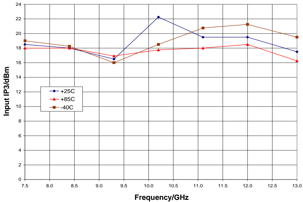
Input IP3 vs. Temperature, LO = +15 dBm, IF = 100 MHz USB
