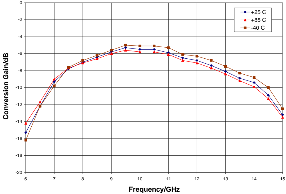
Conversion Gain vs. Temperature, LO = +15 dBm, IF = 100 MHz USB
