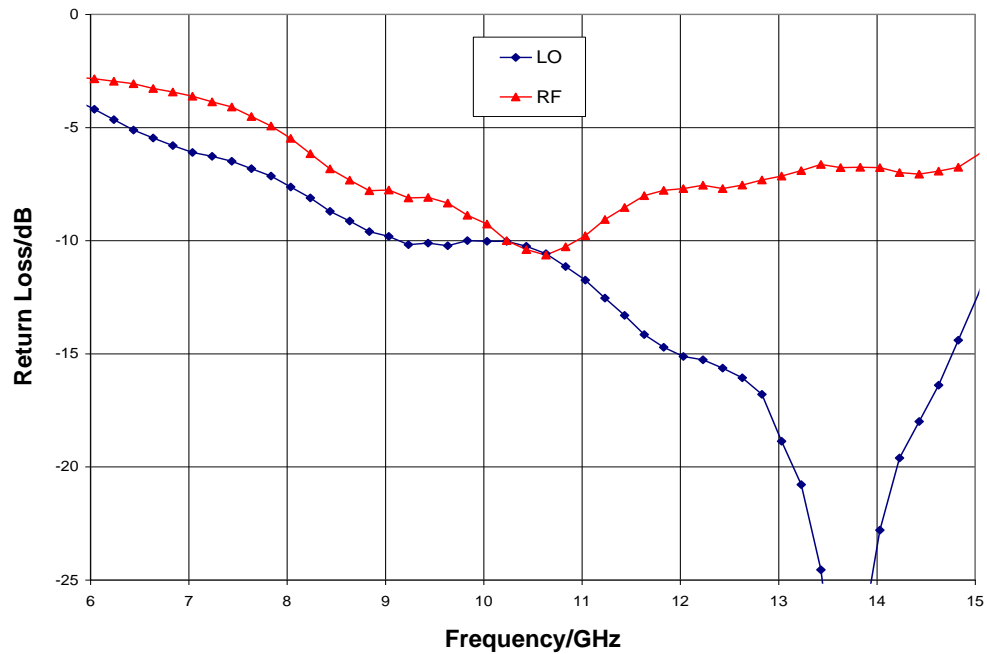
Return Loss, LO = +15 dBm
