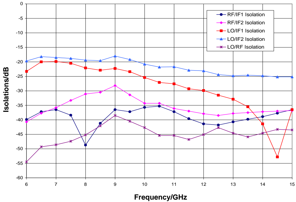
Isolation, LO = +15 dBm. Data Taken Without IF Hybrid
