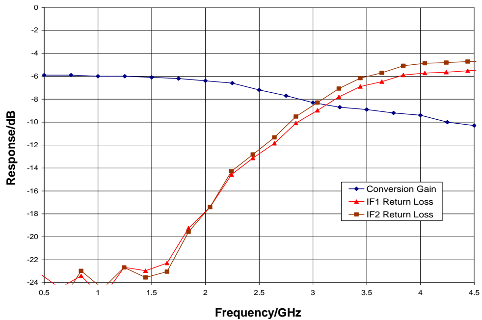
IF Bandwidth, LO = +15 dBm, Return Loss Data Taken Without IF Hybrid
