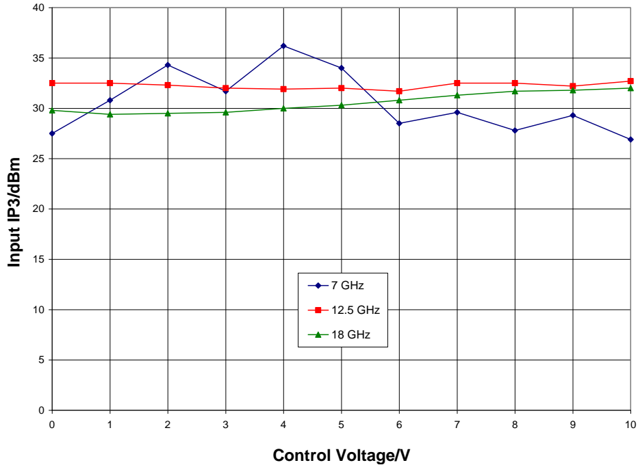
Input IP3 vs. Control Voltage, T_A = 25^\circ\text{ C}
