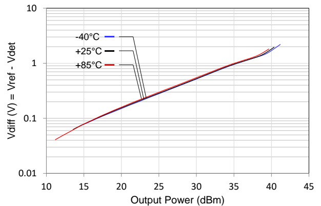
Power Detector vs. Pout vs. Temperature
