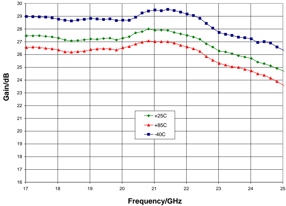
Gain vs. Temperature, V_{dd} = 3.0\text{ V} , V_{gg} = 1.5\text{ V}
