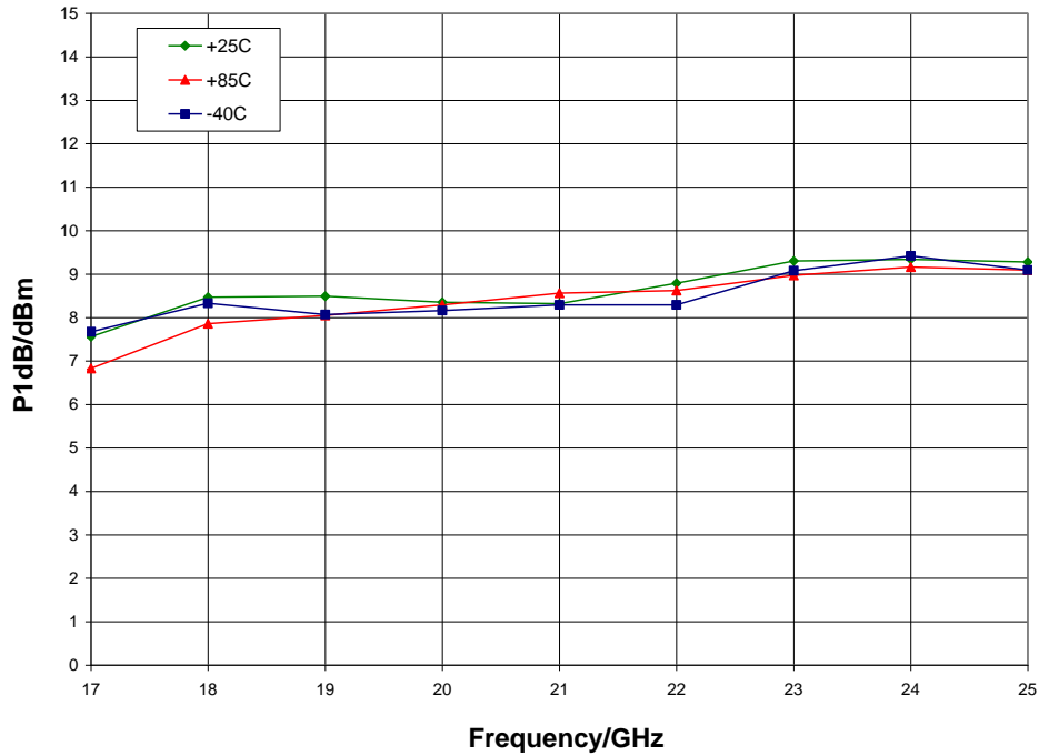
P1dB vs. Temperature, V_{dd} = 3.0\text{ V} , V_{gg} = 1.5\text{ V}
