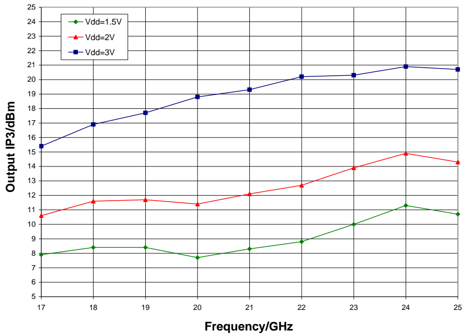
Output IP3 vs. V_{dd} , V_{gg} = 1.5\text{ V} , T_A = 25\text{ °C}
