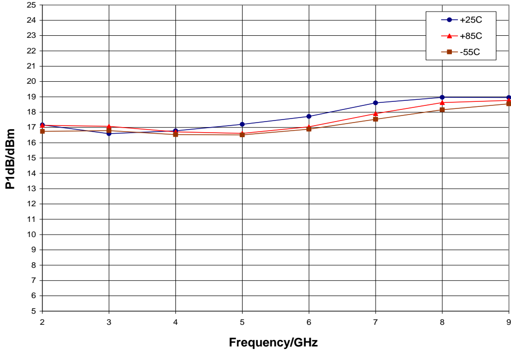
P1dB vs. Temperature, V_{dd} = 6.0\text{ V}
