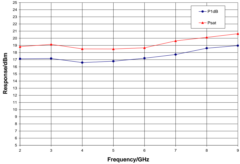
Output Power, V_{dd} = 6.0\text{ V} , T_A = 25\text{ }^\circ\text{C}
