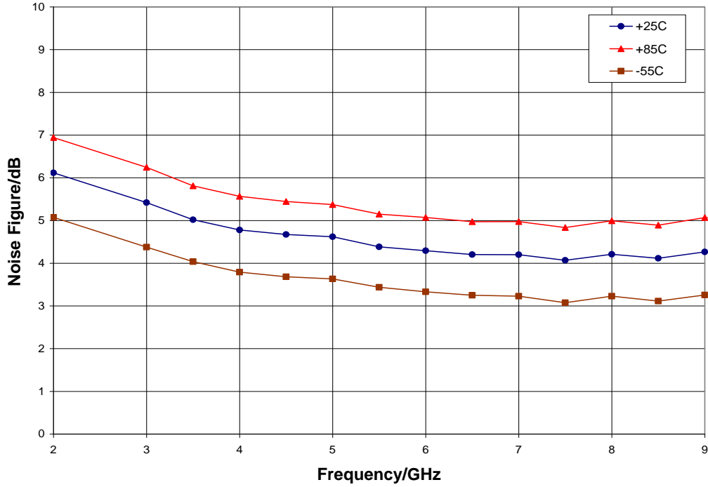
Noise Figure vs. Temperature, V_{dd} = 6.0\text{ V}
