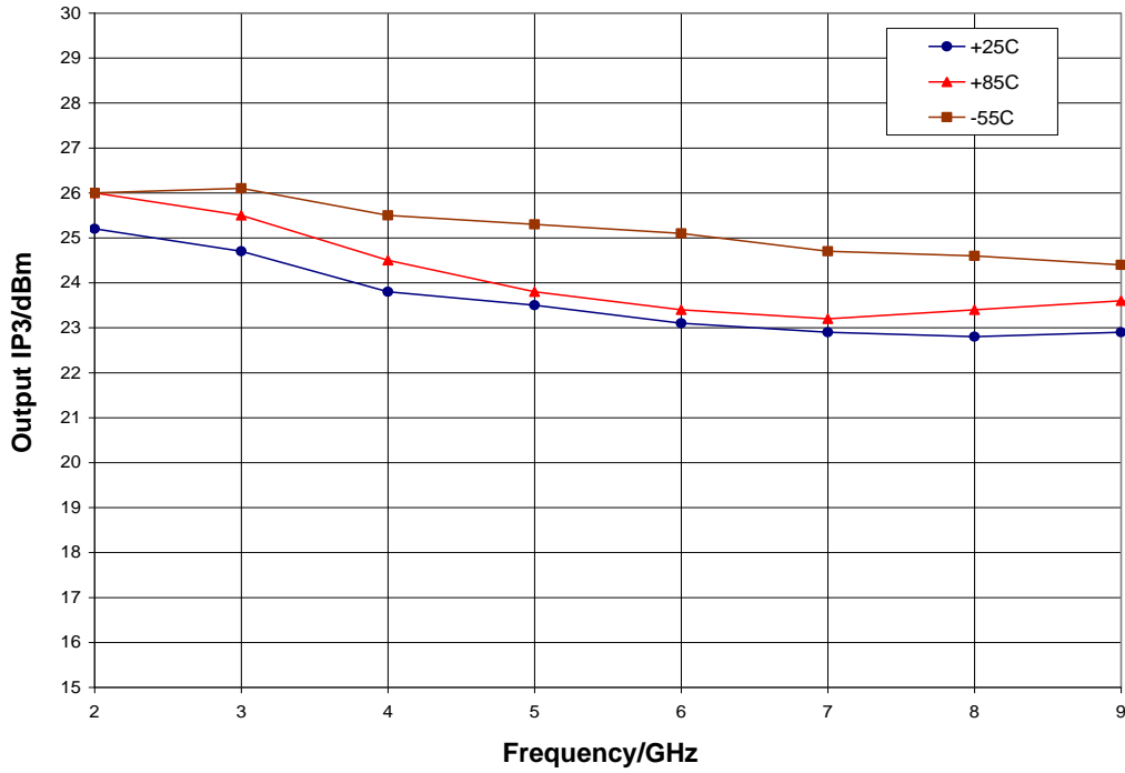
Output IP3 vs. Temperature, V_{dd} = 6.0\text{ V}
