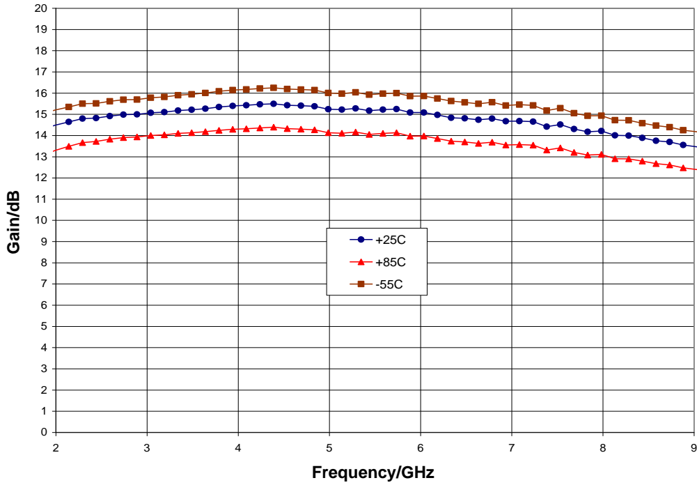
Gain vs. Temperature, V_{dd} = 6.0\text{ V}
