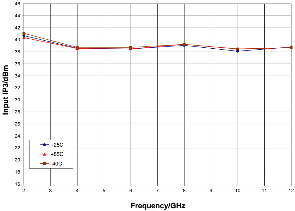
Input Third Order Intercept Point vs. Temperature
