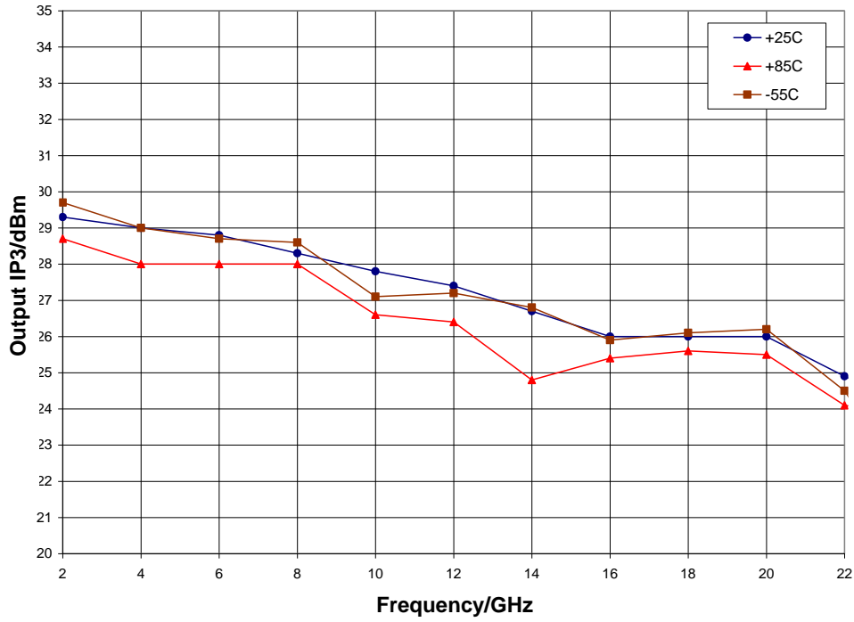
Output IP3 vs. Temperature, V_{dd} = 5\text{ V} , V_{gg} = -0.6\text{ V}
