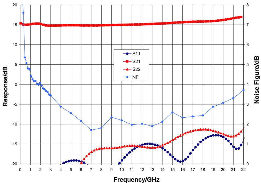
Narrow-band Performance, V_{dd} = 5\text{ V} , V_{gg} = -0.6\text{ V} , I_{dd} = 80\text{ mA} , T_A = 25^\circ\text{ C}
