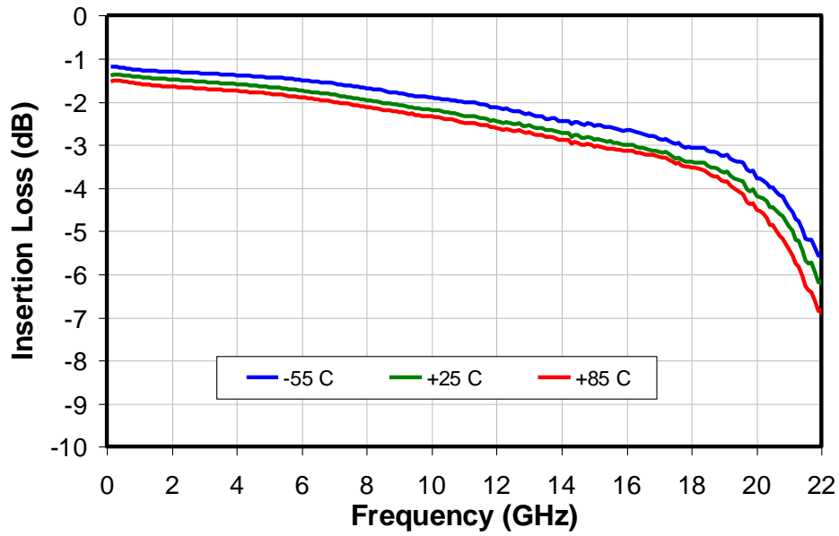
Insertion Loss vs. Frequency
