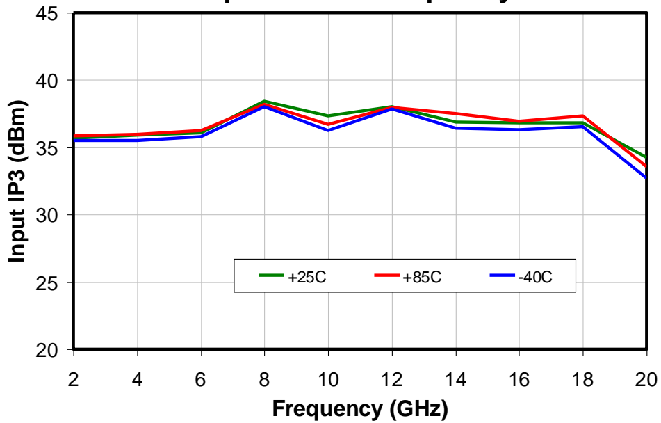
Input IP3 vs. Frequency
