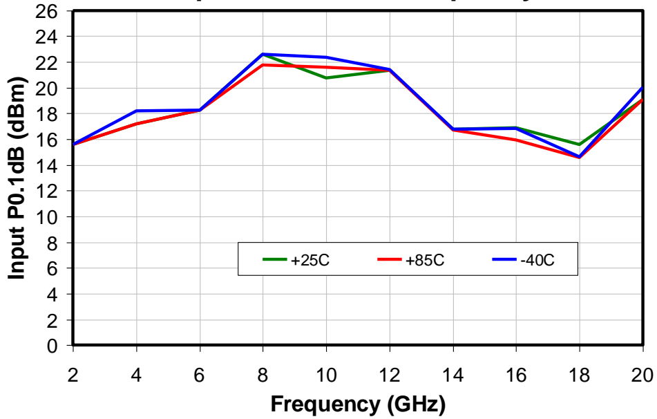
Input P0.1dB vs. Frequency
