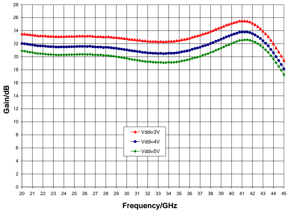
Gain vs. V_{dd} , I_{dd} = 480\text{ mA} , T_A = 25\text{ °C}
