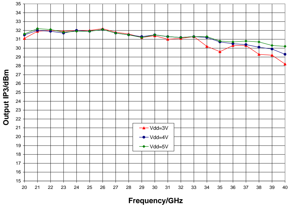
Output IP3 vs. V_{dd} , I_{dd} = 480\text{ mA} , T_A = 25\text{ °C}
