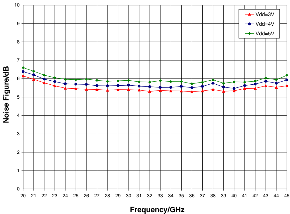
Noise Figure vs. V_{dd} , I_{dd} = 480\text{ mA} , T_A = 25\text{ °C}
