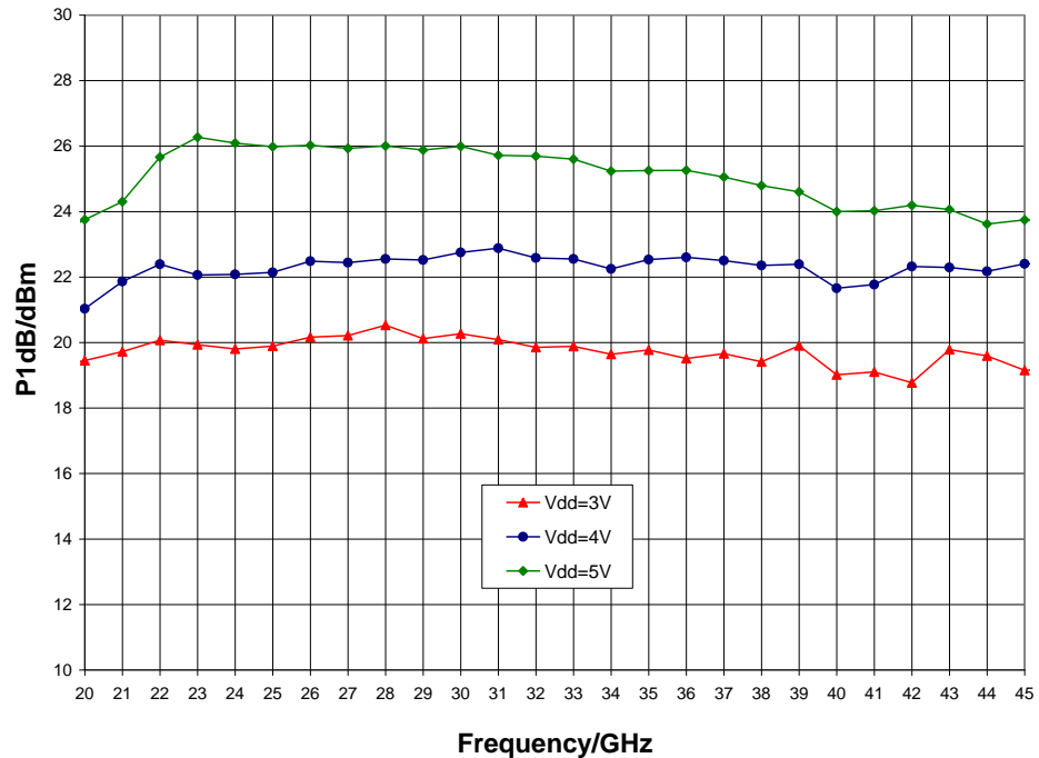
P1dB vs. V_{dd} , I_{dd} = 480\text{ mA} , T_A = 25\text{ °C}
