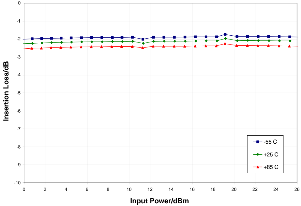
Insertion Loss vs. Pin @ 18 GHz, V_{ctl} = 0\text{ V}
