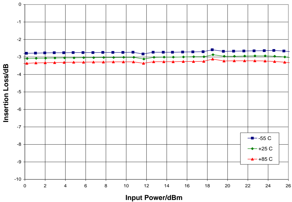
Insertion Loss vs. Pin @ 12 GHz, V_{ctl} = 0\text{ V}
