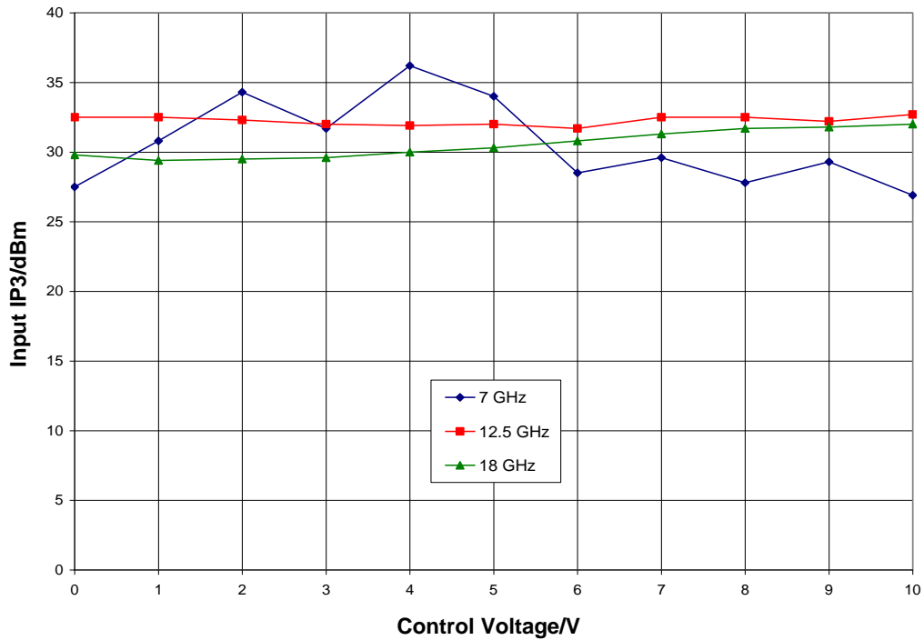
Input IP3 vs. Control Voltage, T_A = 25\text{ °C}
