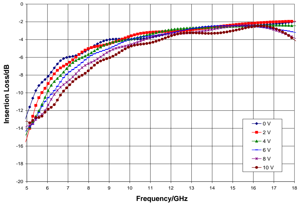
Insertion Loss vs. Frequency, T_A = 25\text{ }^\circ\text{C}
