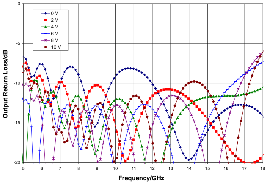
Output Return Loss, T_A = 25\text{ }^\circ\text{C}
