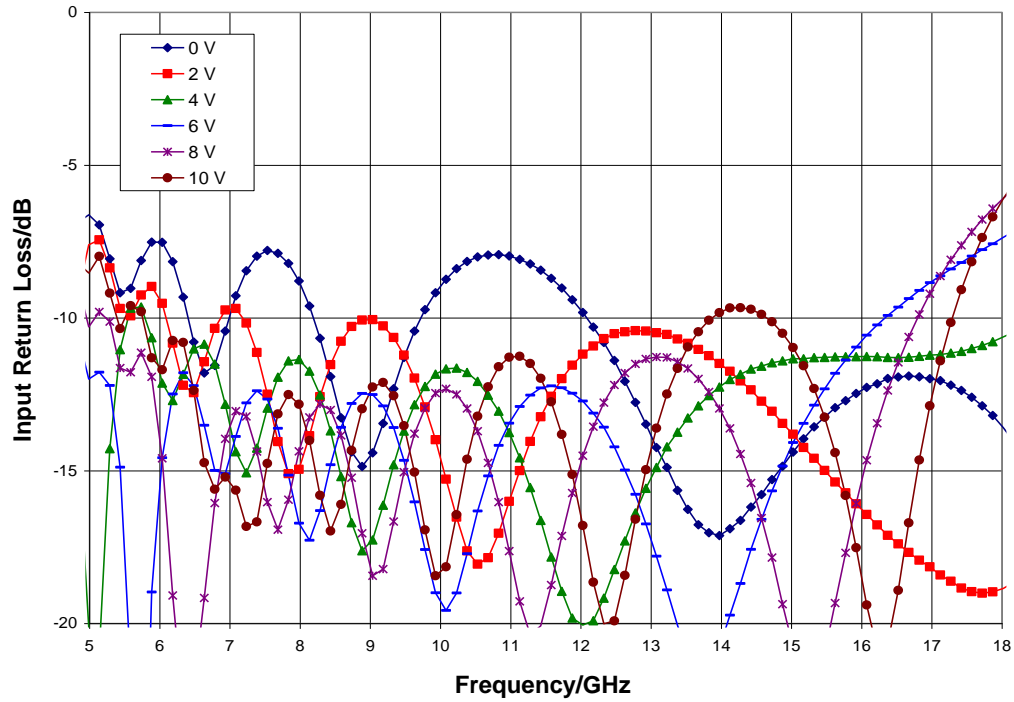
Input Return Loss, T_A = 25\text{ }^\circ\text{C}
