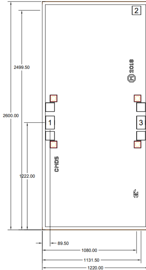
Die Outline (all dimensions in microns)
