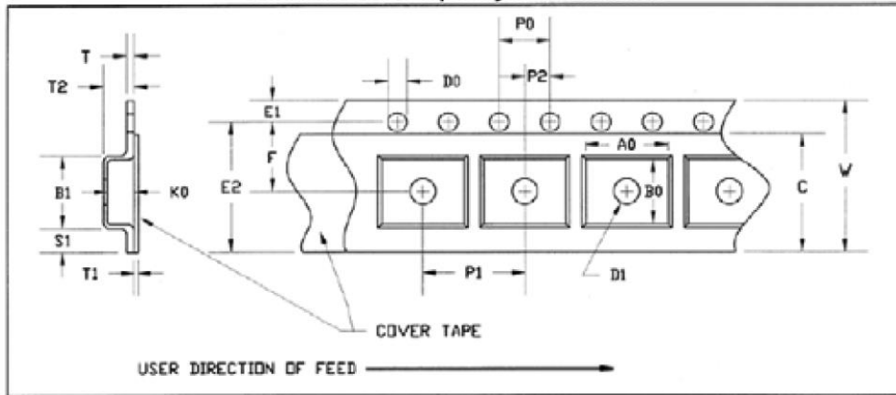
Carrier and Cover Tape Physical Dimensions
