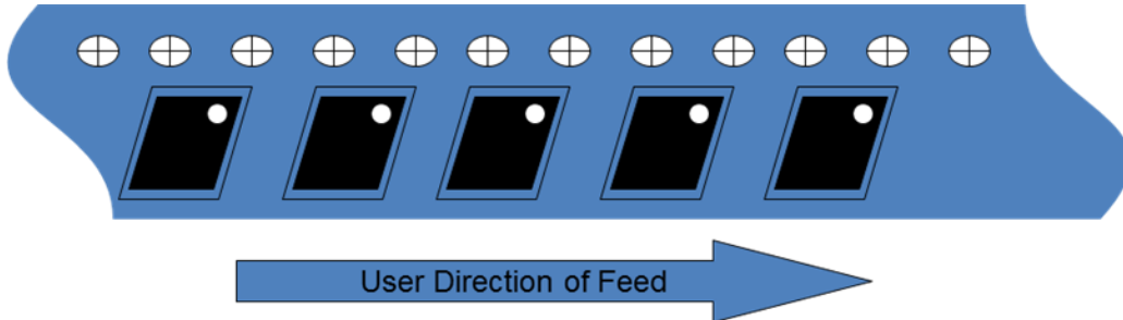
Carrier and Cover Tape Physical Dimensions
