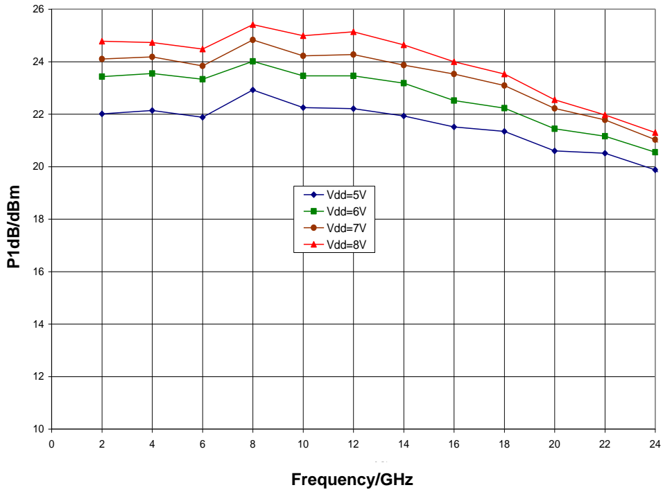
P1dB vs. Supply Voltage, T A = 25 °C
