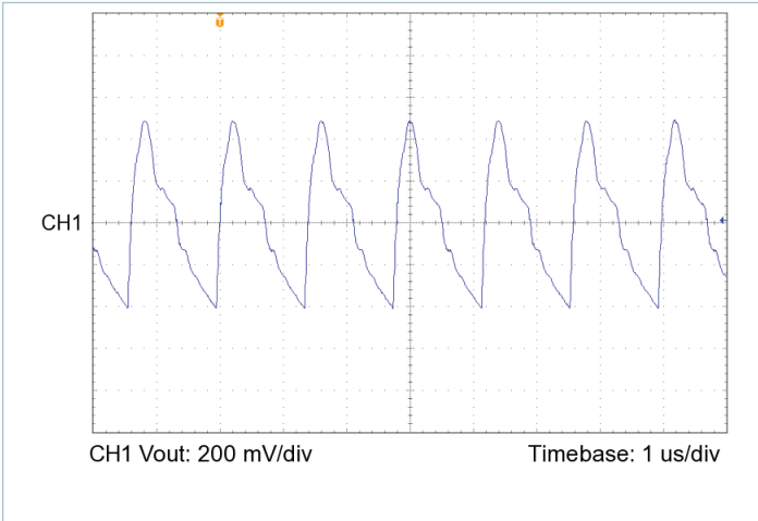
Figure 18 — Output voltage ripple, V_{IN} = 28\text{V} , V_{OUT} = 48.0\text{V} , C_{OUT\_EXT} = 200\mu\text{F} , R_{LOAD} = 7.200\Omega
