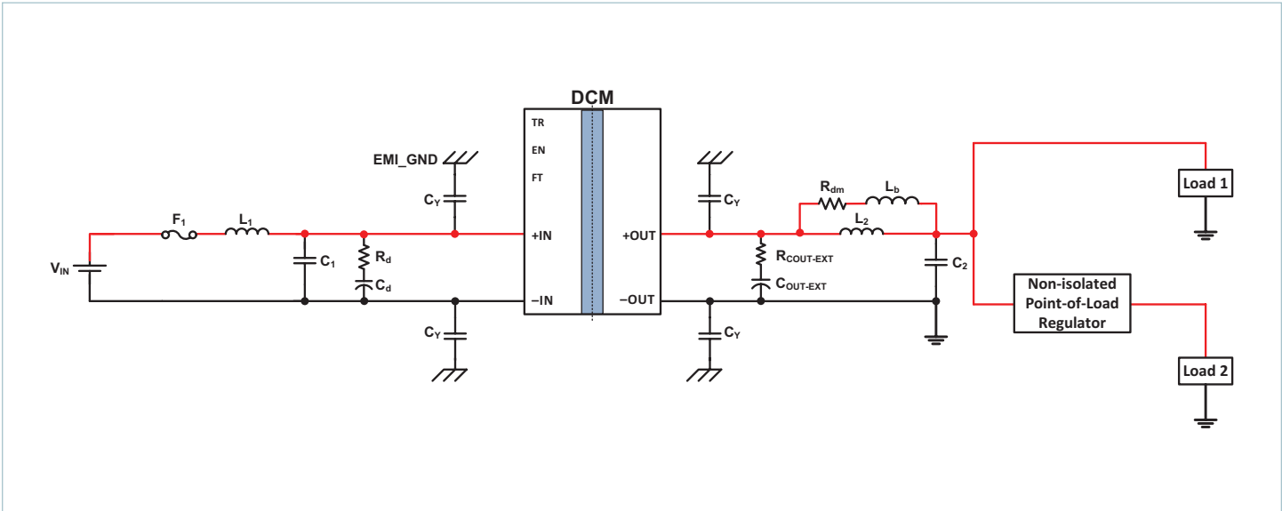
Typical application 1: single DCM3623x50M53C2y7z to a non-isolated regulator and direct to load
