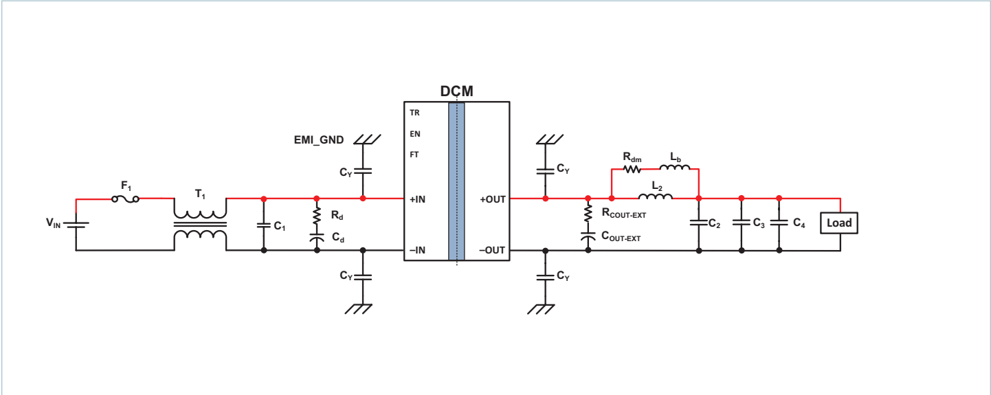
Typical application 2: single DCM3623x50M53C2y7z with common- and differential-mode input filters
