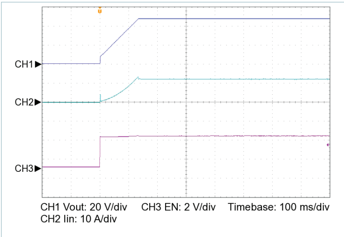
Figure 19 — Start up from EN, V_{IN} = 28\text{V} , C_{OUT\_EXT} = 2000\mu\text{F} , R_{LOAD} = 7.200\Omega
